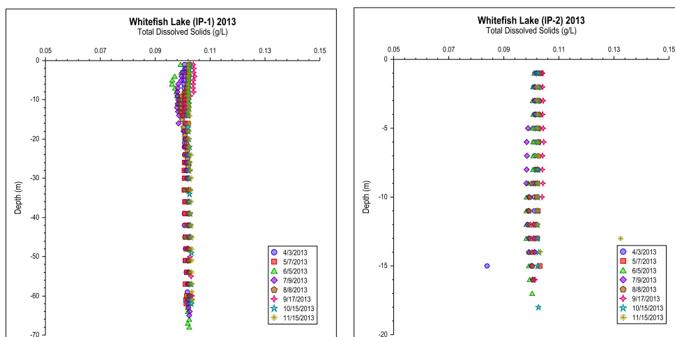
Figure 98. Typical Seasonal TDS Pattern Two Sites 2013.
