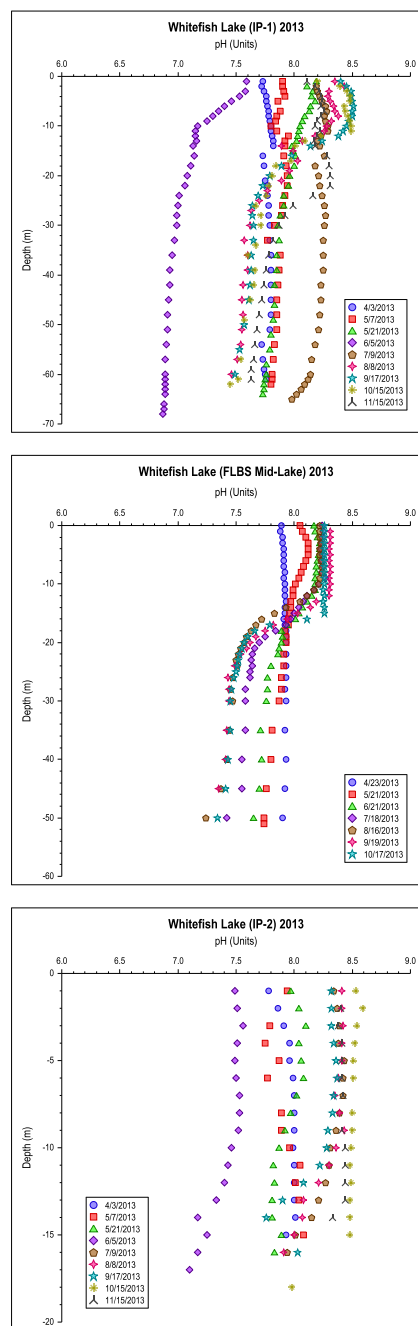
Figure 96. Typical Seasonal pH Pattern Three Sites 2013.
